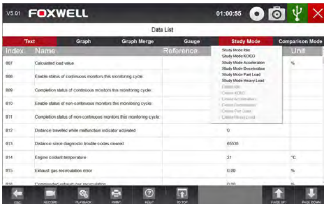
Figure 4-32 Sample Study Mode Screen
