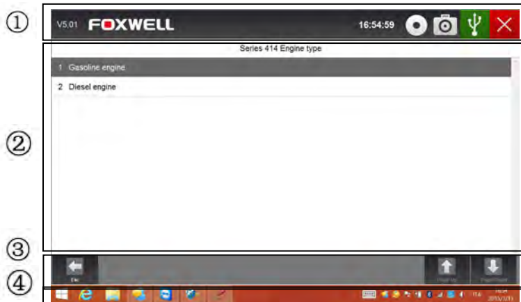
Figure 4-1 Title Bar
